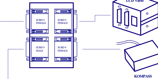
485 Splitting Unit (using additional LCD vario and Kompass)
