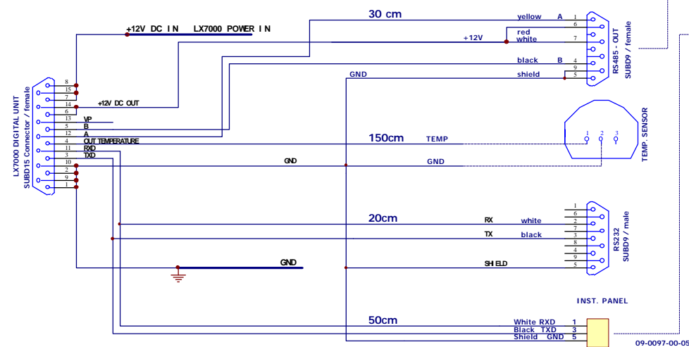
LX7000 / LX20 Communication Cable (delivery not included)
